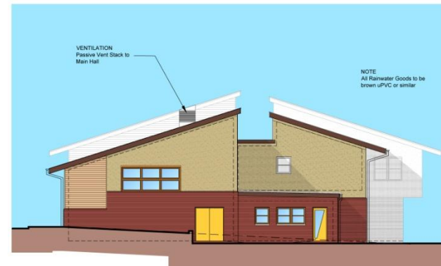
North Elevation
